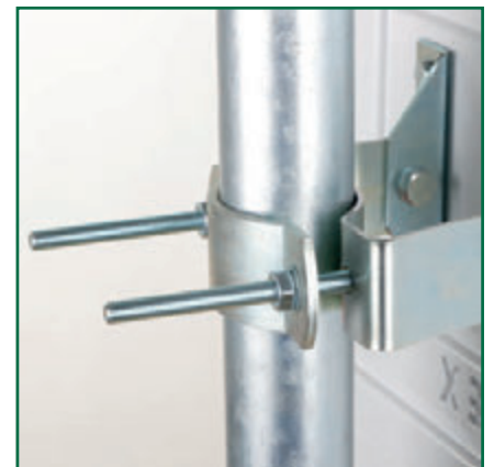
Photo: Back side with standard post fixing
