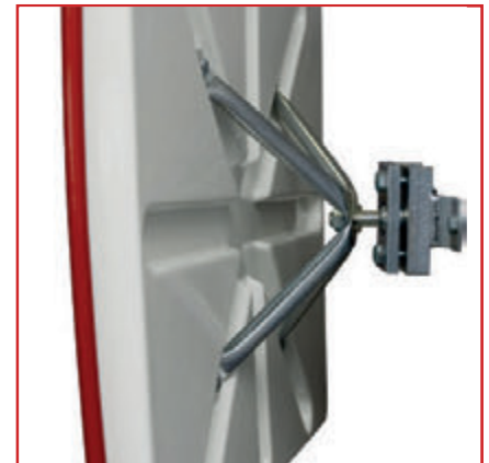
Photo: Back side: 4-point fixing with ball joint for an optimal fixation
